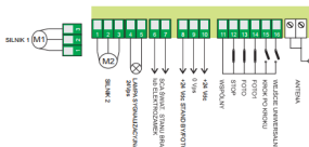
WING02024/WING03524 (MC424L)
