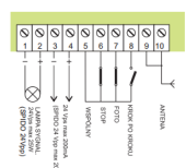
WIDE (WIA2)
